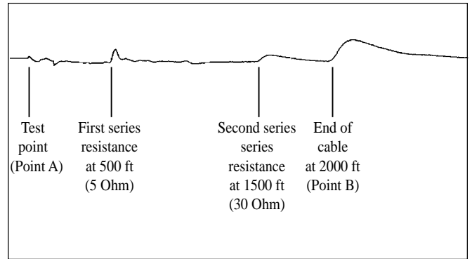
Description of test setup, measuring from the near end.
