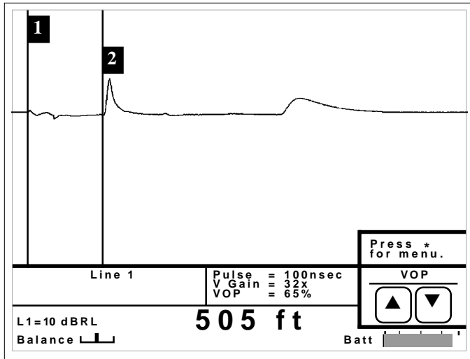
Measuring from the far end.
